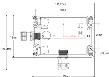
XT4* -BCL Boîtier IP65 polyester chargé
